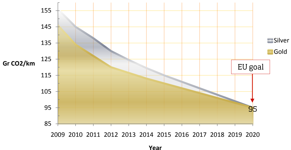
The reduction path to the 2020 goal of 95 gr CO 2 /km
